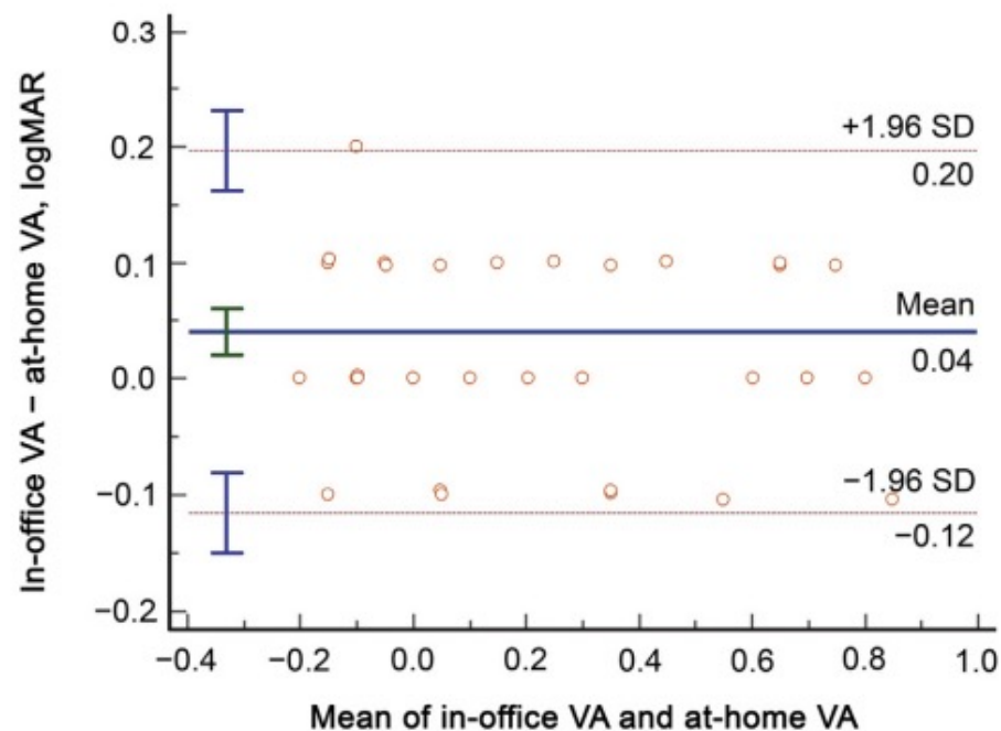
FIG 2. Bland-Altman plot comparing E-ETDRS visual acuity test results obtained in office and at home for 31 children (62 eyes) 7-12 years of age.
