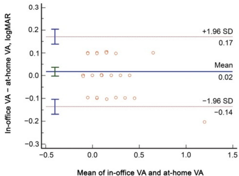
FIG 1. Bland-Altman plot comparing ATS-HOTV visual acuity test results obtained in office and at home for 34 children (68 eyes) 3-6.9 years of age.
